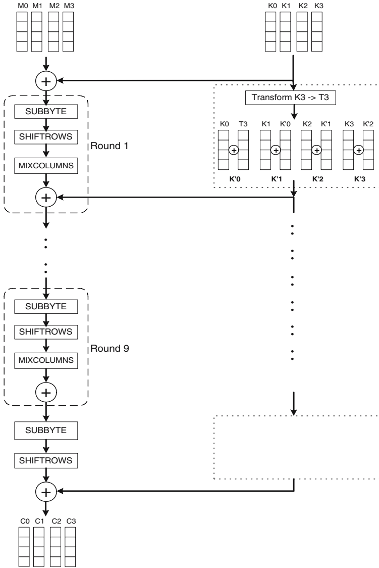
Fig. 2. AES structure
