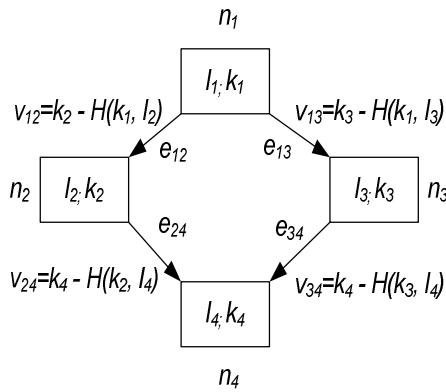
Fig. 2. Key scheme proposed in [21] which is the basis for the multiple access control of our DRM system. The arithmetic is modulo \rho which is a proper number.
