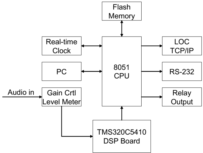
Fig. 5. System structure
