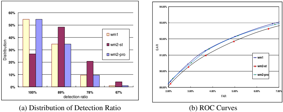
Fig. 6. Comparison of the Proposed Dual Watermarking(wm2-pro) with the Straightforward Dual Watermarking(wm2-st)
